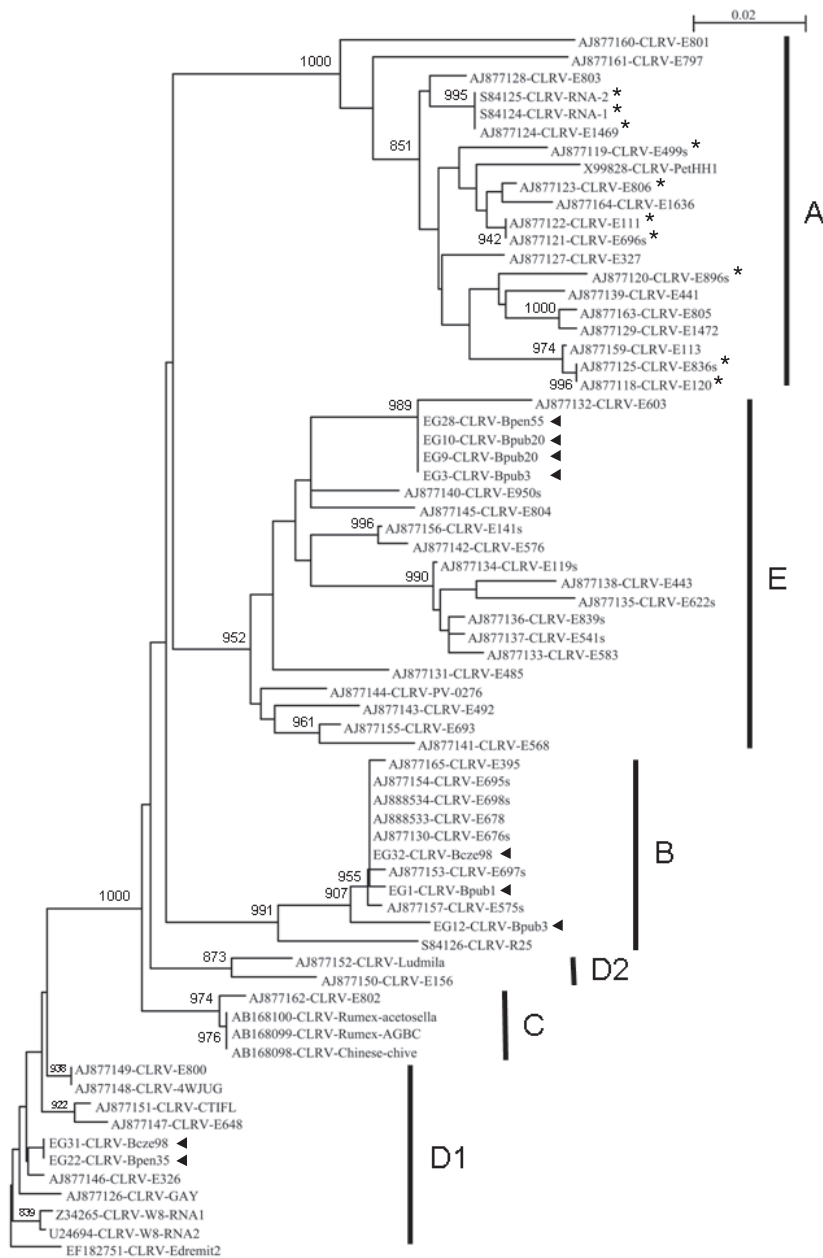
Fig. 3. Phylogenetic tree inferred from the nucleotide sequence alignment (386 bp) of the 3' non-coding regions of Cherry leaf roll virus isolates generated with ClustalX 1.83 applying the neighbour-joining algorithm. Bootstrap analysis was performed with 1000 repetitions and values above 800 are indicated at branch nodes. The scale bar of 0.02 represents 2 nucleotide substitutions per 100 nucleotides of the aligned sequences. Sequences obtained from the NCBI database are indicated by their accession numbers according to Table 1. CLRV sequences obtained from Betula spp. in Finland (Table 3) are indicated with arrowheads, isolates originating from Betula spp. in Germany and United Kingdom are pinpointed with asterisks. Phylogenetic groups (A to E) according to Rebenstorf et al. (2006) are indicated by bold lines on the right.
