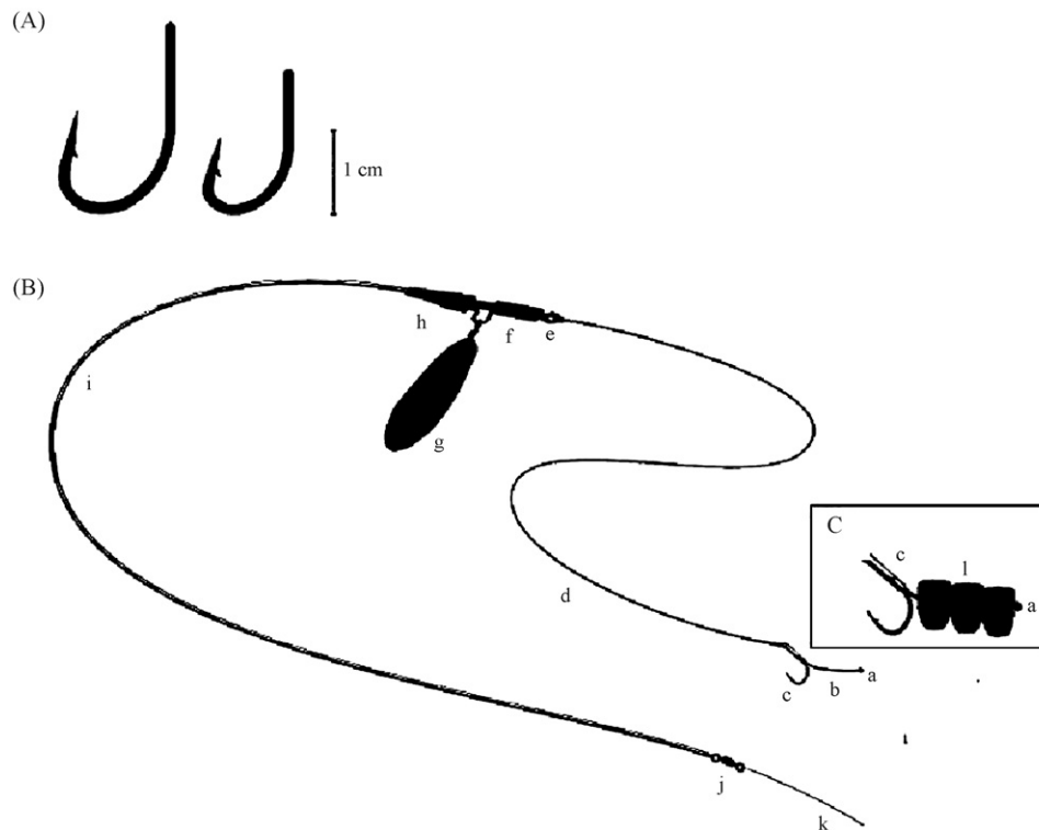
Fig. 1. Illustrations of the hook sizes used in the present study (plot A), the rig used in this study (plot B) and the hair baited with corn (plot C): (a) boilie stopper, (b) hair, (c) hook, (d) leader, (e) swivel, (f) clip, (g) lead sinker, (h) rubber, (i) braided line with a lead core, (j) swivel, (k) braided main line, and (l) corn.
